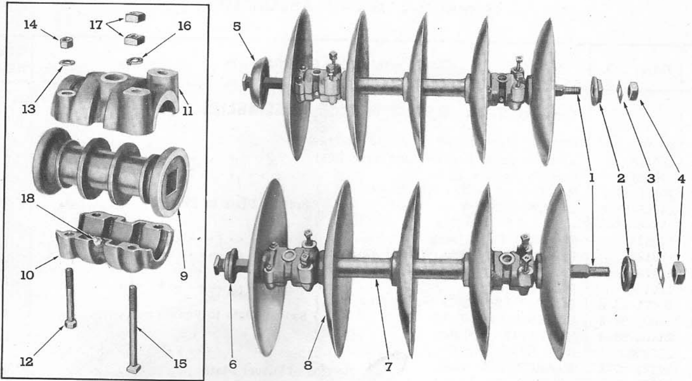
Figure 12 - Disc and Bearing Assemblies
