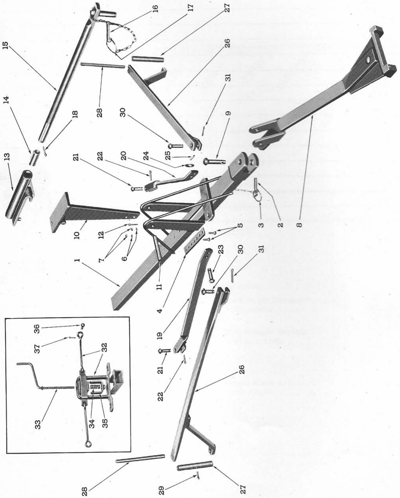
Figure 10 - Hitch and Lever Angling Assemblies
