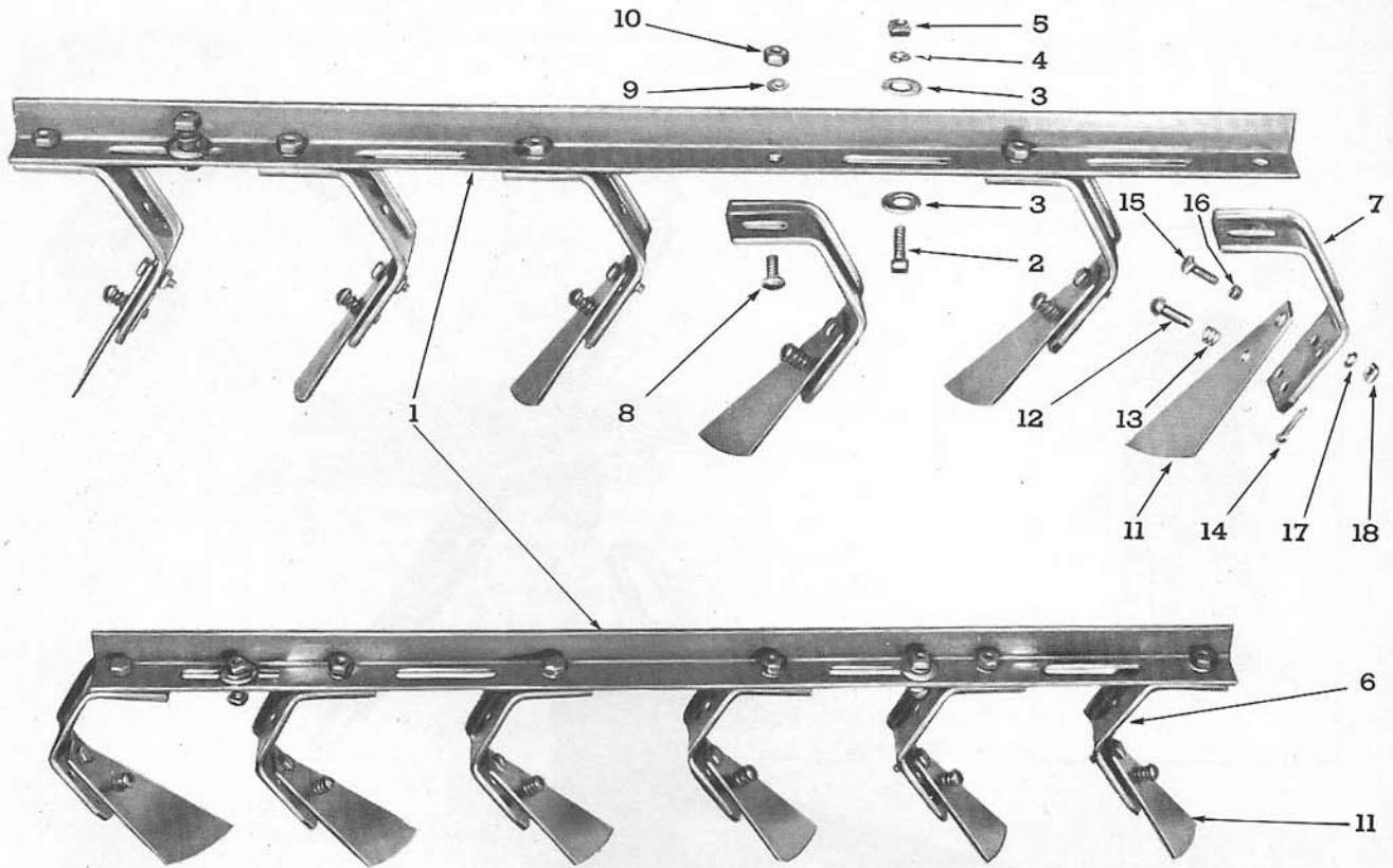
Figure 13 - Scraper Assemblies
